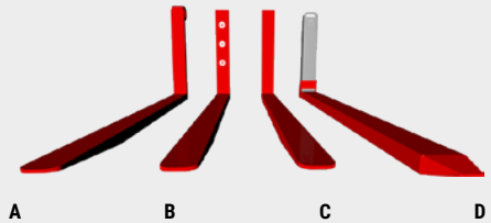
A - PIN-TYPE FORKS B - BOLTED FORKS
